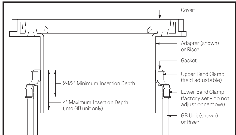
Figure 2 - Insertion Depths
