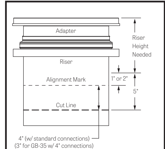
Figure 1 - Riser Measurements
